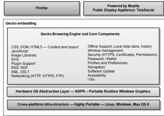
Figure 4: Overview of Gecko infra-structure and kiosk application which brings Web content
