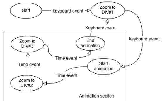
Figure 5: Diagram with keyboard event interruptions between occurrences of the guided tour animation
