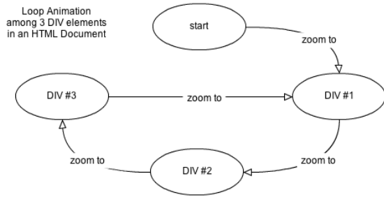
Figure 3: A state diagram for a sequential loop animation among DIV elements
