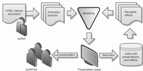
Figure 6: Visual narrative meta-data builds an index system and facilitates the reuse presentation assets
