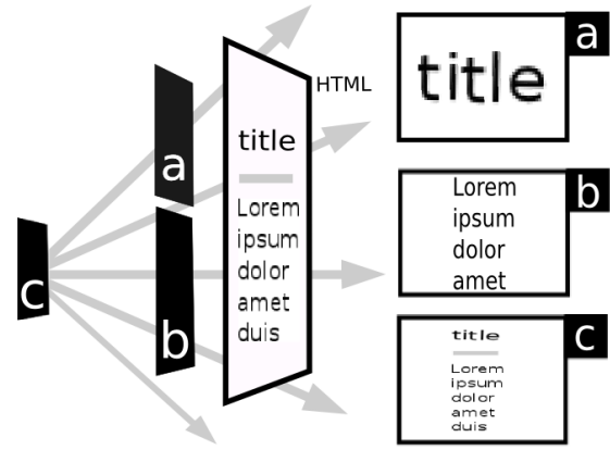
Figure 1: A, B, and C are possible viewports. A to B can be achieved with panning but C involves pan and zoom out
